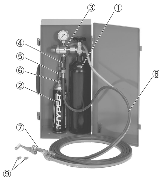
TA370TD-N
